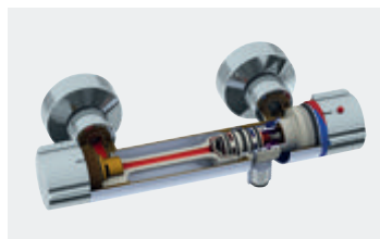
H9769 cut-away: low water volume, thermal insulation and no non-return valves Ref. DELABIE: Coupe3D_H9769
